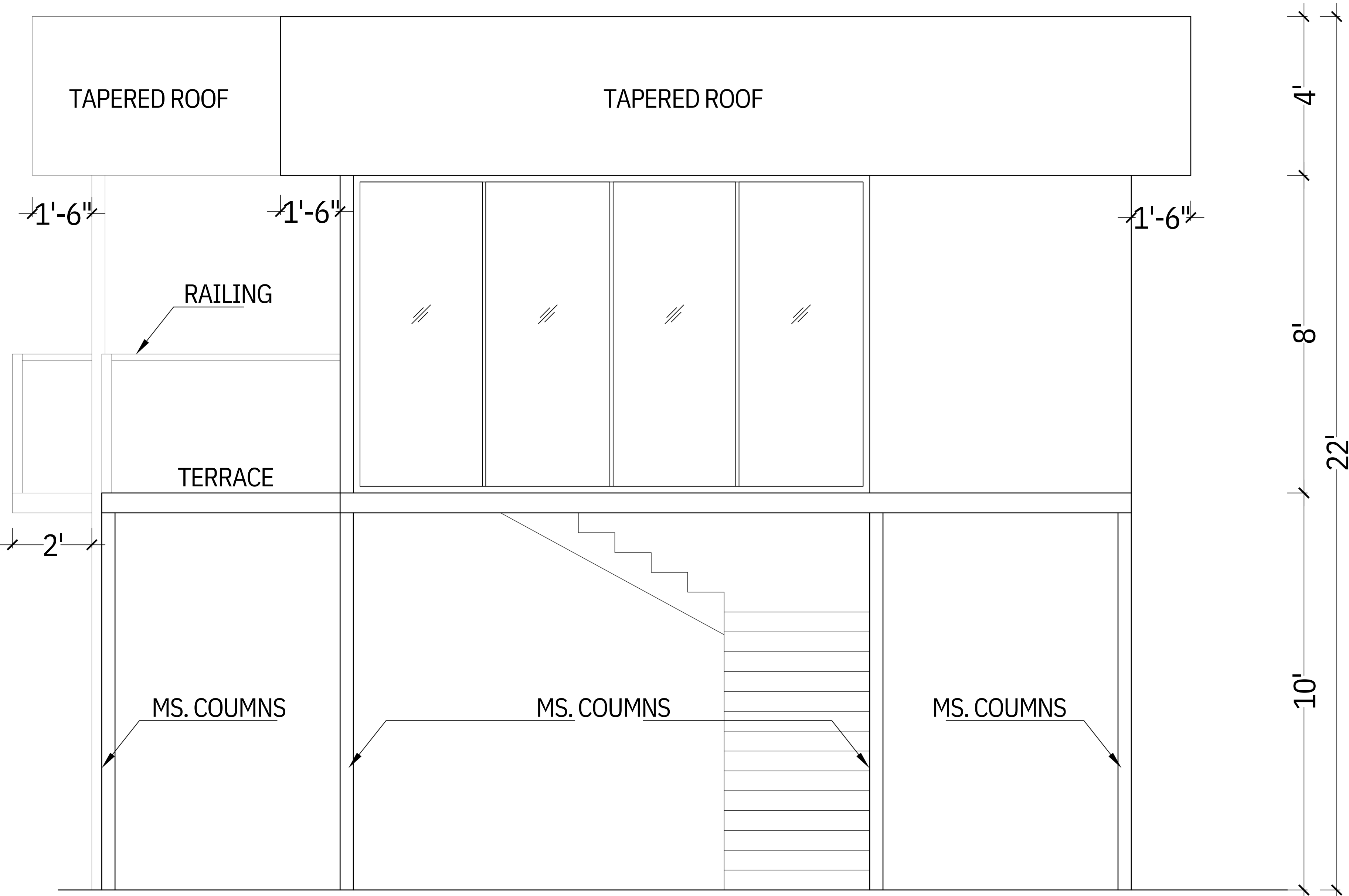
LEFT SIDE ELEVATION
