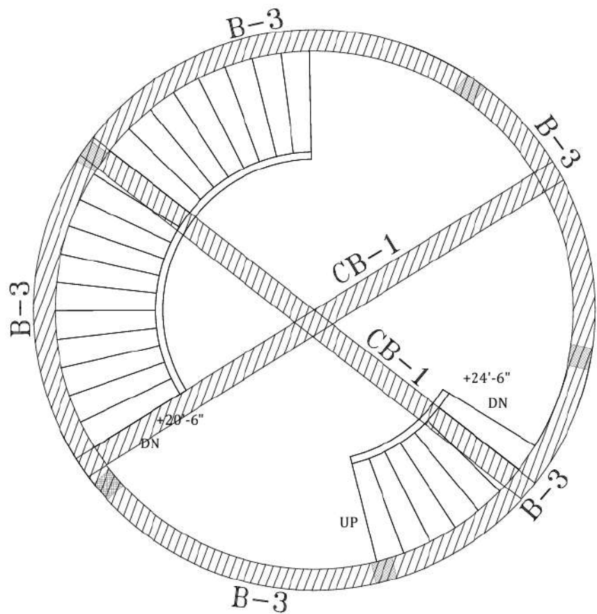
(COUPLING BEAM AT 20'-0" LEVEL)
