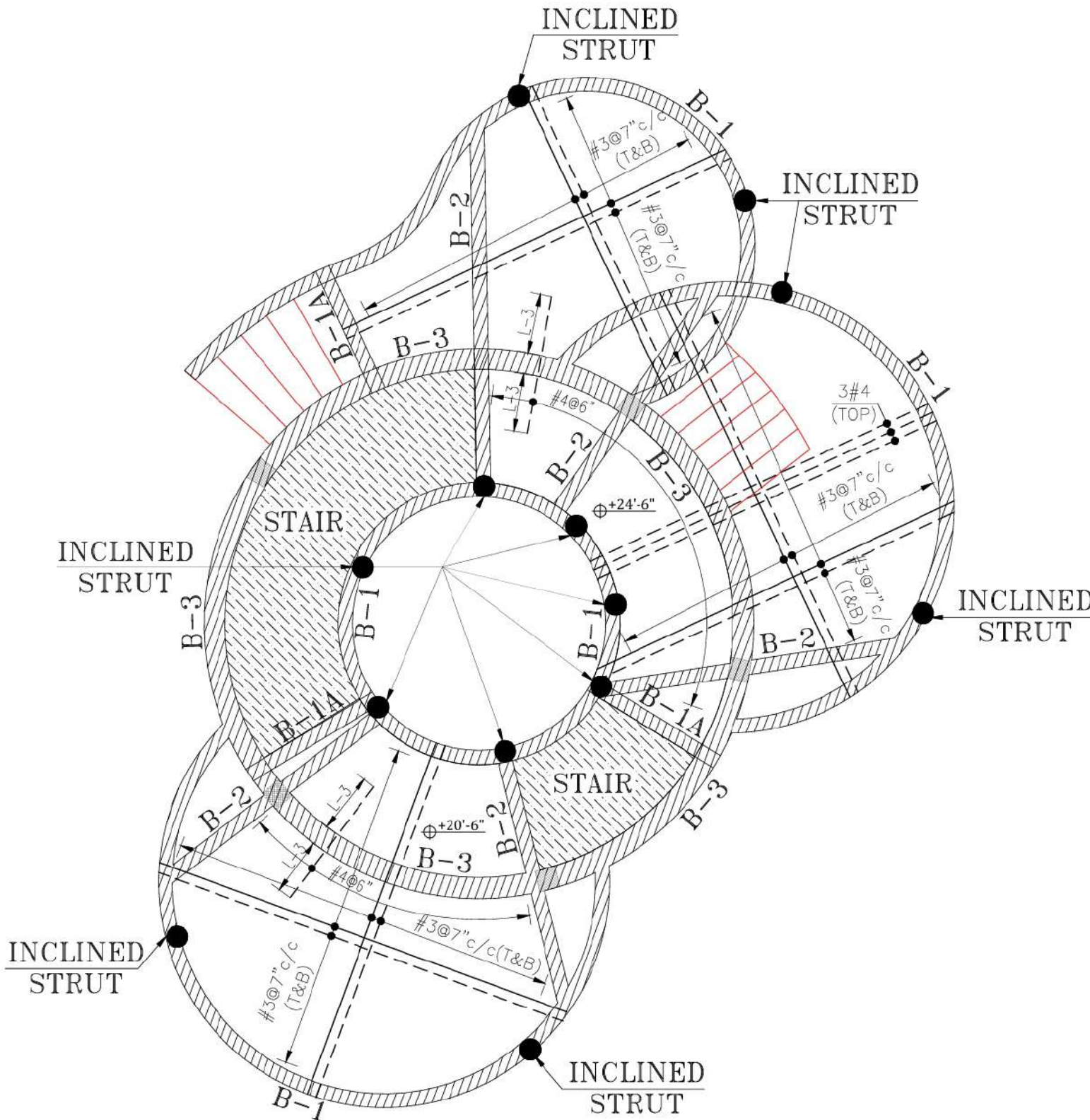
FIRST FLOOR-ROOF SLAB ALL SLABS 6" THICK
