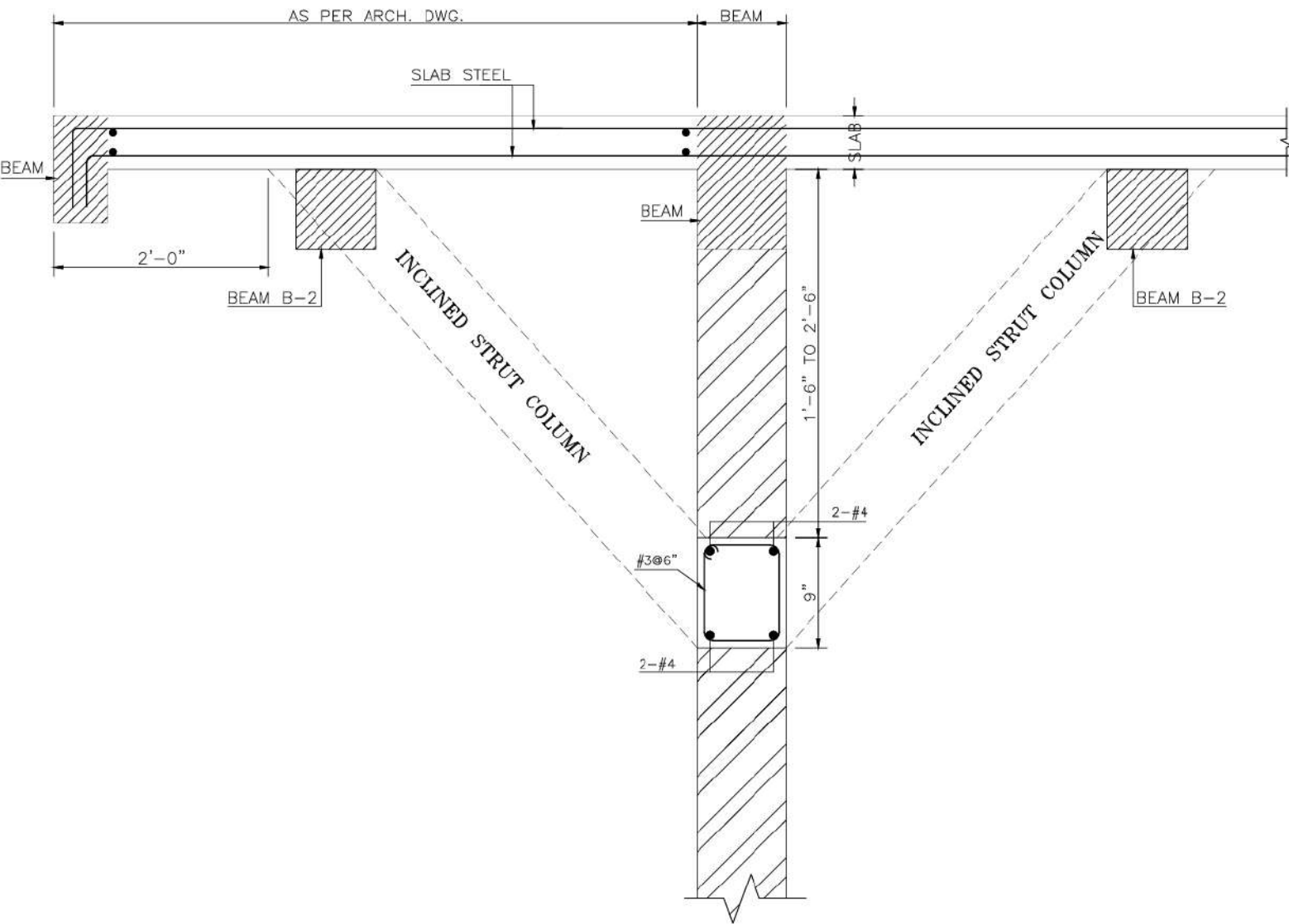
TYPICAL STRUT COLUMN DETAIL
