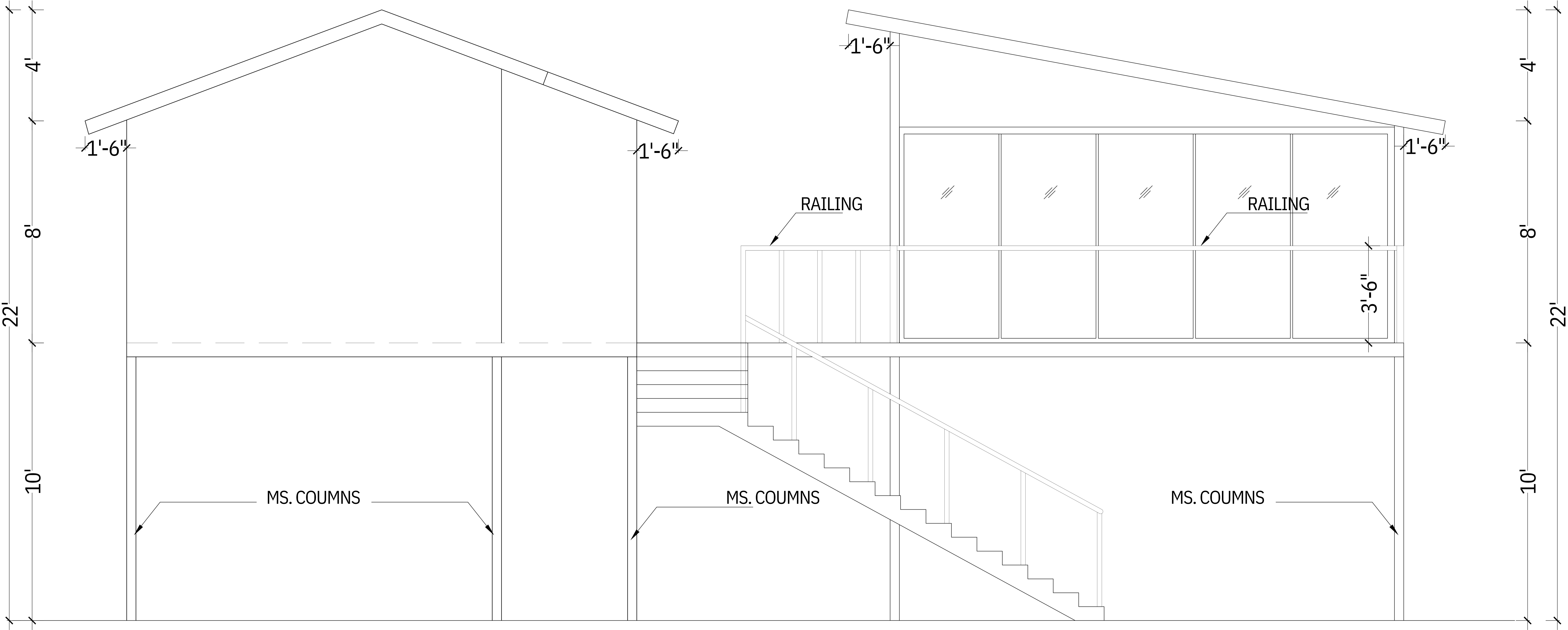
FRONT SIDE ELEVATION
