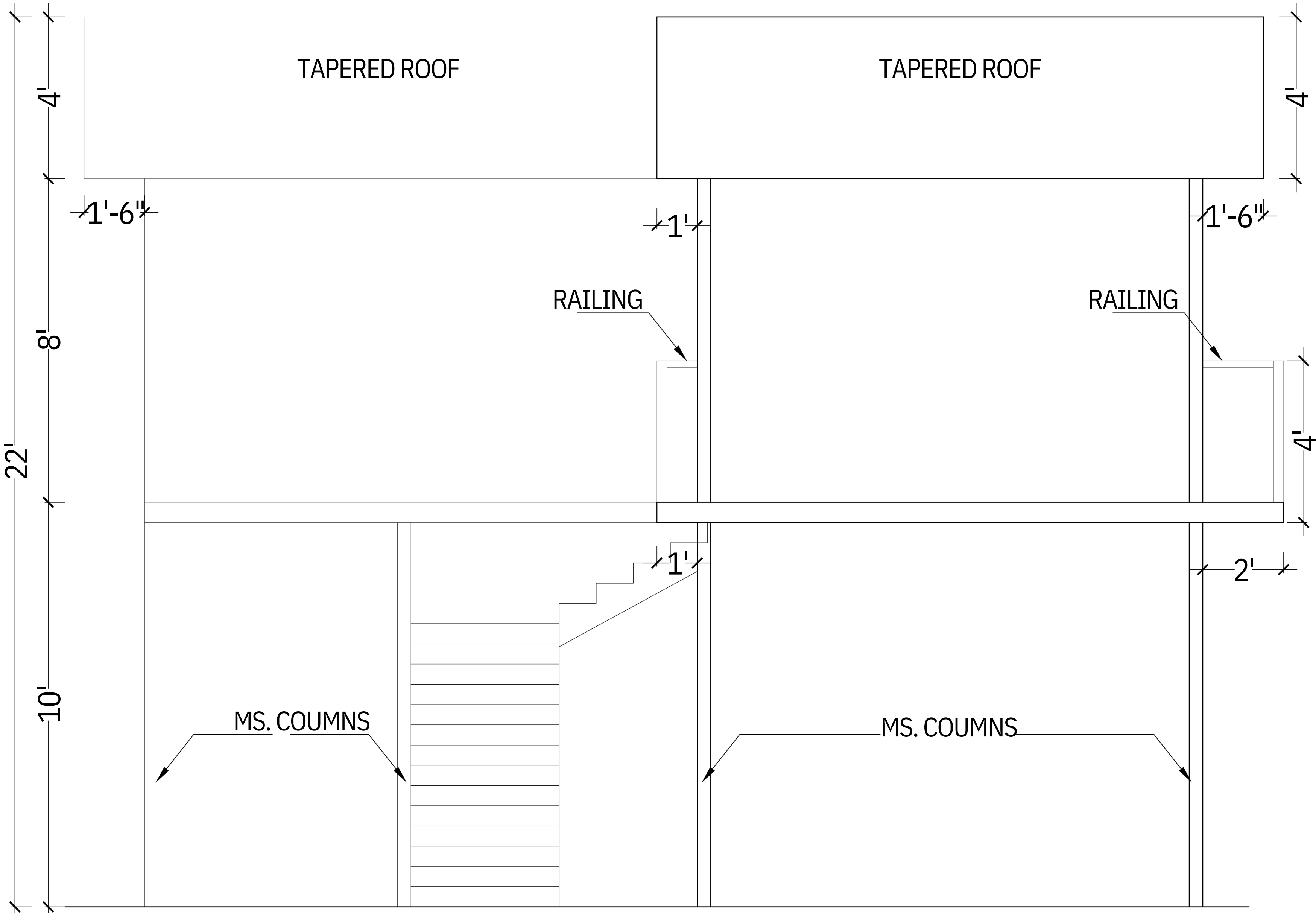
RIGHT SIDE ELEVATION
