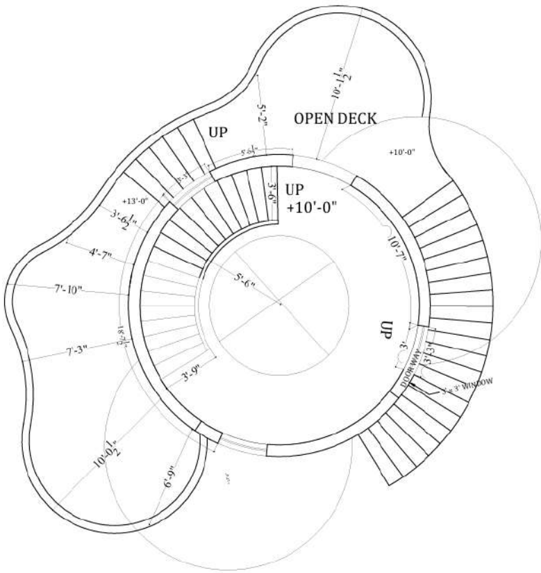
LEVEL 1 PLAN
