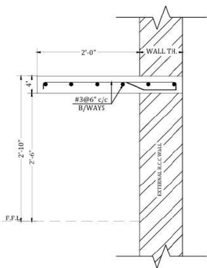
S-03 REINF. DETAIL FOR SLAB AT 34" Scale: 3/4"=1'-0"
