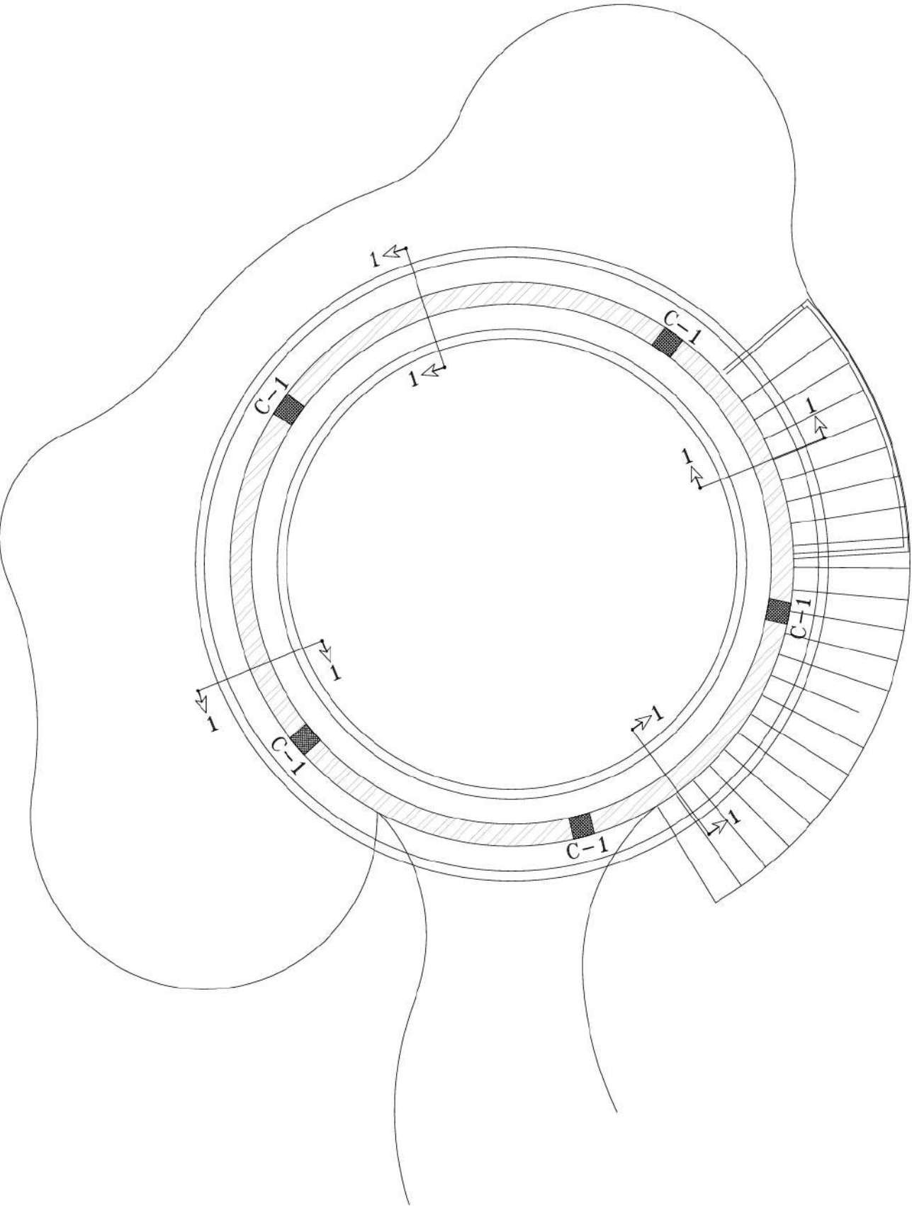
FOUNDATION PLAN
