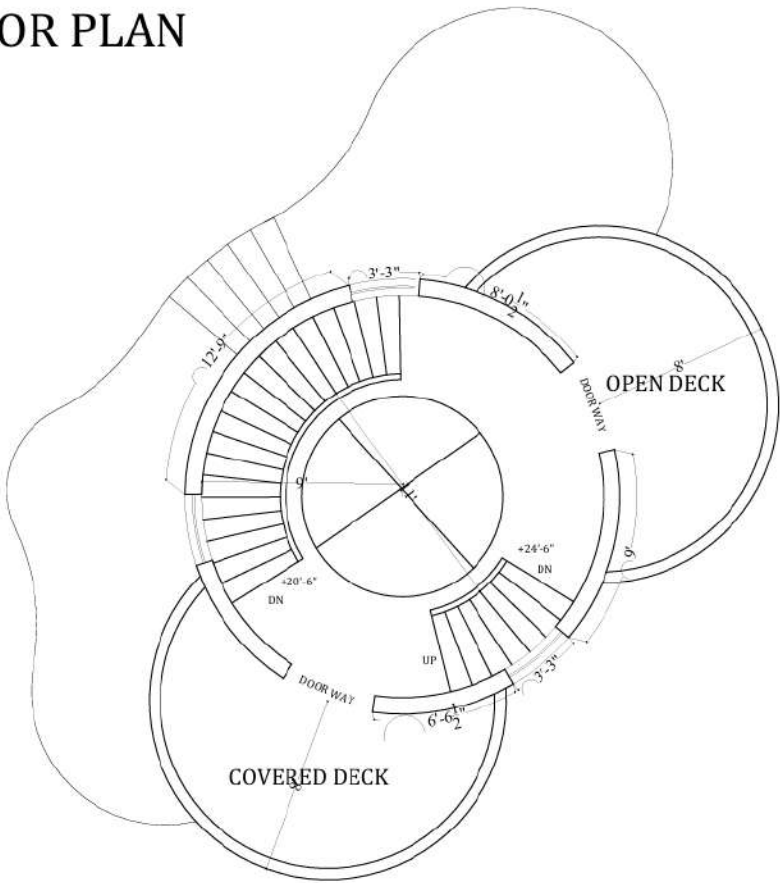
LEVEL 2 PLAN
