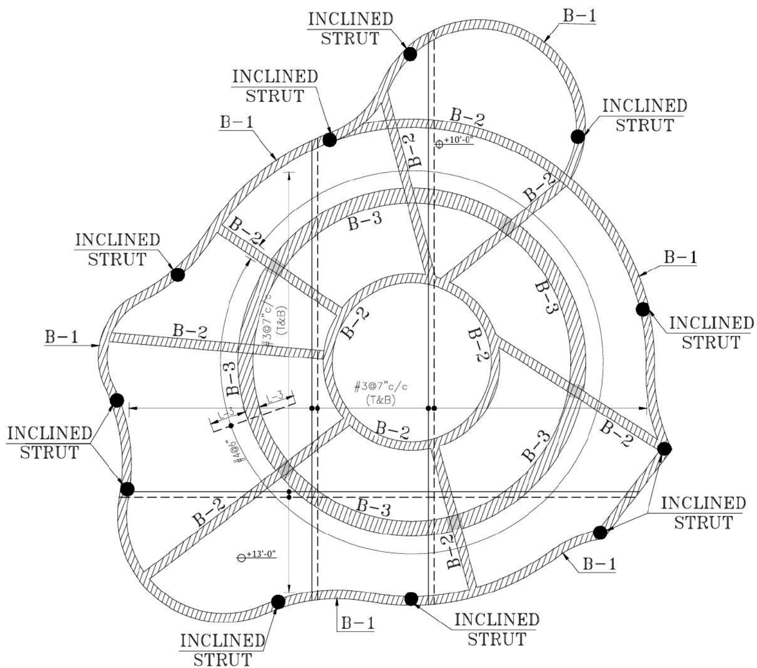
GROUND FLOOR-ROOF SLAB ALL SLABS 6" THICK
